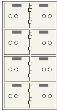
AXN-8 (Wt. 86 lbs.) 8 openings ea. 5" x 5"
